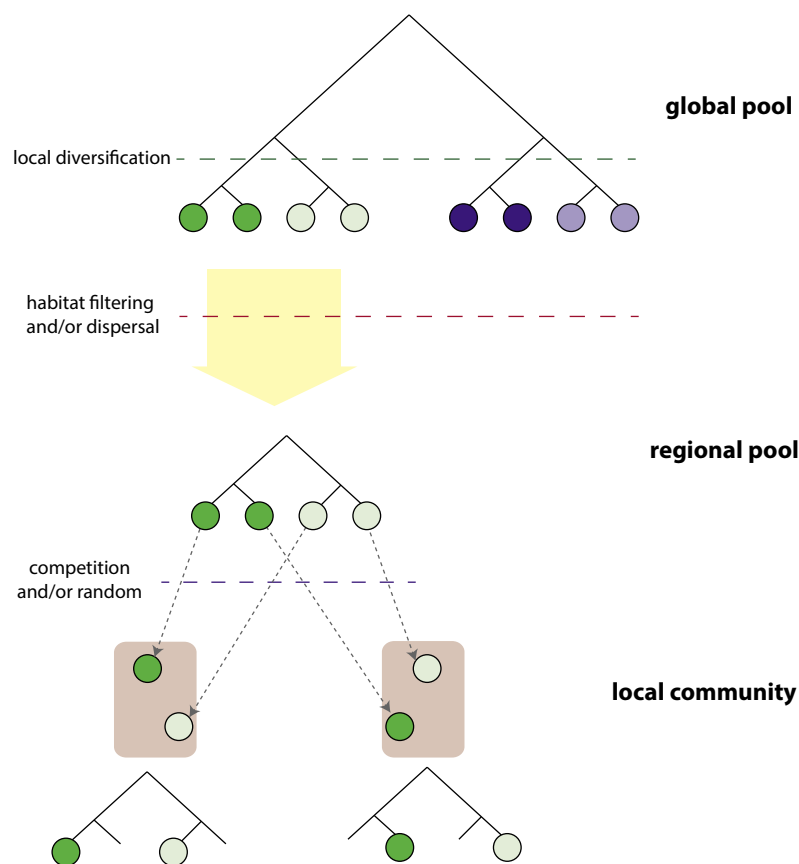
Figure 4. Schematic diagram illustrating an assembly model of the Graphis scripta complex community, based on the current findings.
